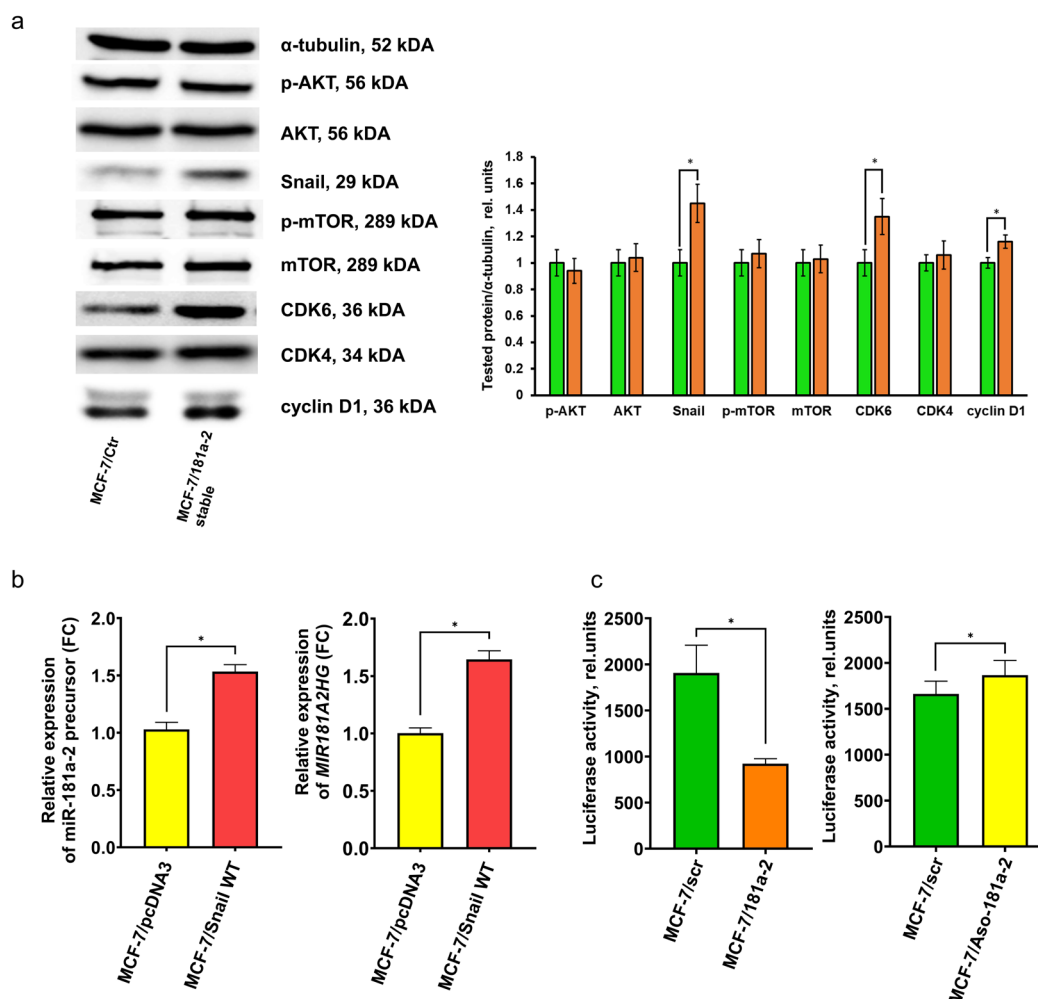
Figure 4. (a) Western blot analysis of growth-related proteins in MCF-7/Ctr and MCF-7/miR-181a-2 cells. The blot shows results representative of three independent experiments; t-test, *P=0.034 for Snail, 0.035 for CDK6, 0.045 for cyclin D1 (b) expression of cellular miR-181a-2 precursor (left panel, *P value=0.0005, unpaired t test) and MIR181A2HG (right panel, *P value=0.0002, unpaired t test) in MCF-7 cells following wtSnail transfection, data are presented as mean \pm SD ( n=3 ); (c) reporter assay of E-cadherin transcriptional activity in the cells after transfection of scrambled miR/miR-181a-2 (left panel, *P value=0.0007, unpaired t test) and after transfection of antisense (Aso) DNA oligonucleotides scrambled/Aso-miR-181a-2 (right panel, *P value=0.0398, unpaired t test), data are presented as mean \pm SD ( n=3 )
